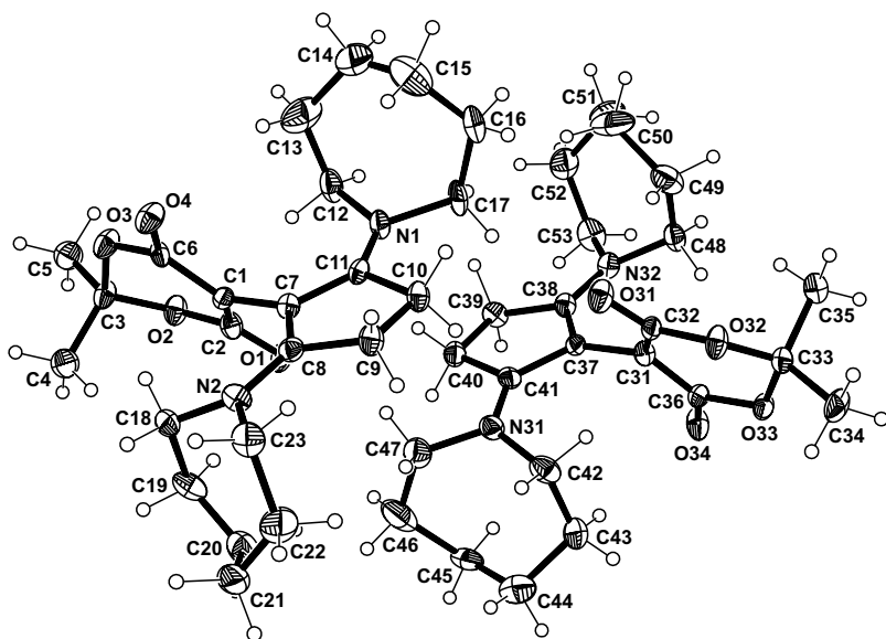
FIG. 4 The molecular structure of 10 with the 30% probability ellipsoids
